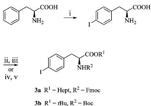
Scheme 2. Reagents and conditions: i) I 2 , NaIO 3 , H 2 SO 4 /AcOH, 70 °C, NaIO 4 , 87%; ii) heptanol, TsOH, 80 °C, 53%; iii) NaHCO 3 then FmocOSu, dioxane, 86%; iv) Boc 2 O, NaOH, dioxane, 90%; v) t BuBr, K 2 CO 3 , n Bu 4 NBr, DMAC, 93%.
